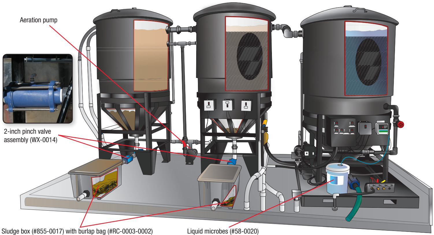
Sludge box (#855-0017) with burlap bag (#RC-0003-0002)
